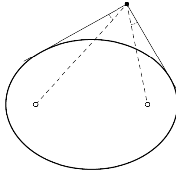
11.5) Poncelet's theorem
